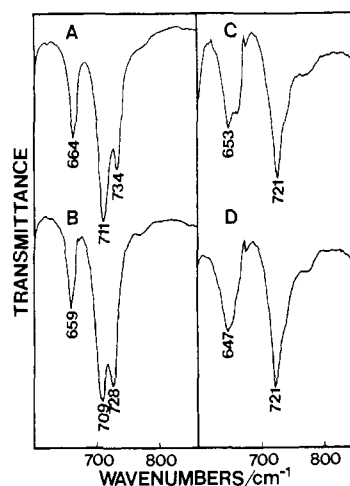
Figure 2. Infrared spectra of solid-state (A) glycylglycine, (B) [1- 13 C]glycyl[ 15 N]glycine, (C) glycylglycine methyl ester, and (D) [1- 13 C]glycyl[ 15 N]glycine methyl ester.
