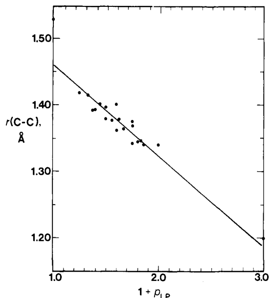
Figure 5. Experimental data for the C-C bond distances, r(\text{C-C}) in angstroms plotted as a function of the \sigma -bond order plus Pauling \pi -bond order 1 + p_{LP} . The straight line conforms to the linear least-squares fit r(\text{C-C}) = -0.136(1 + p_{LP}) + 1.597 \text{ \AA} . The standard deviation in r(\text{C-C}) is 0.019 \text{\AA} , and the correlation coefficient r^2 = 0.8762 .
